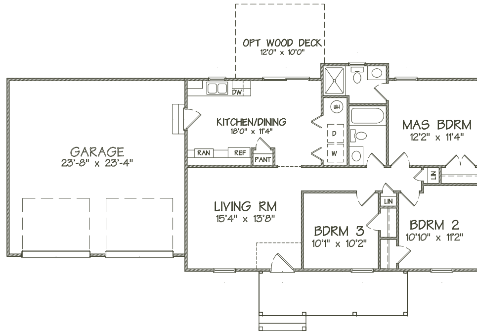
FLOOR PLAN
