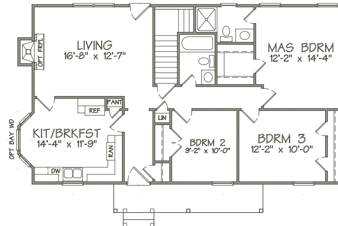
FLOOR PLAN W/BASEMENT
