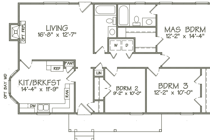
FLOOR PLAN W/CRAWL SPACE
