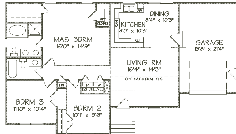
FLOOR PLAN WITH CRAWL SPACE
