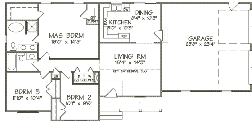
FLOOR PLAN WITH CRAWL SPACE
