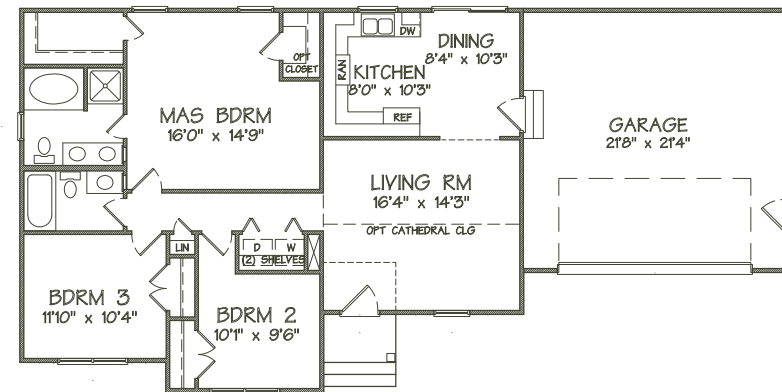
FLOOR PLAN WITH CRAWL SPACE
