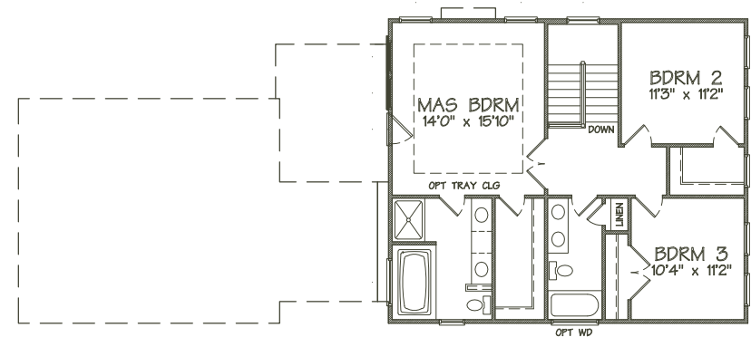
UPPER LEVEL FLOOR PLAN
