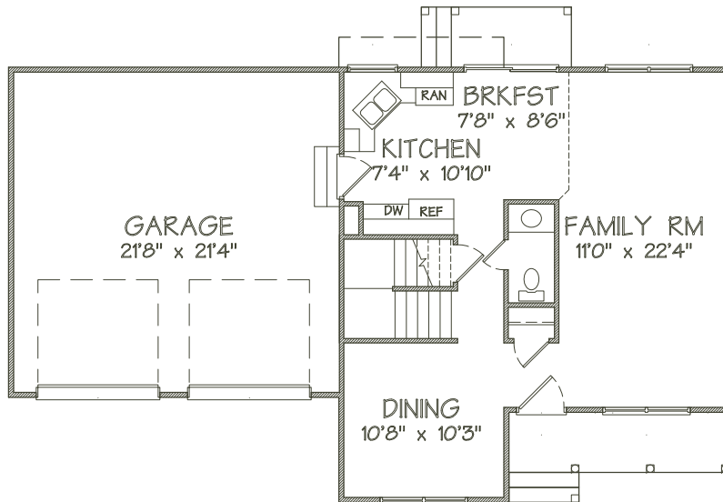
LOWER LEVEL FLOOR PLAN
