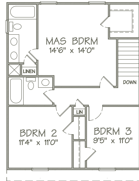
UPPER LEVEL FLOOR PLAN
