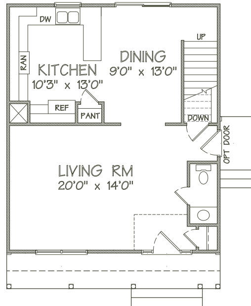
LOWER LEVEL FLOOR PLAN
