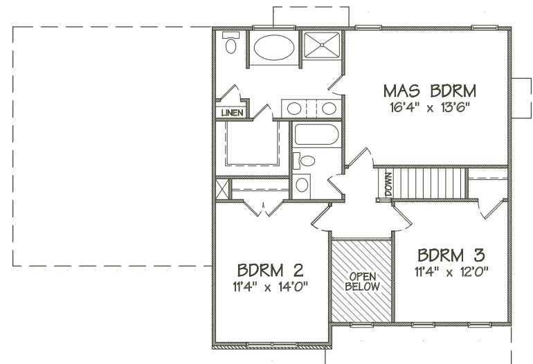
UPPER LEVEL FLOOR PLAN
