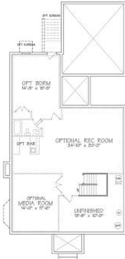
BASEMENT PLAN 1106 SQ FT
